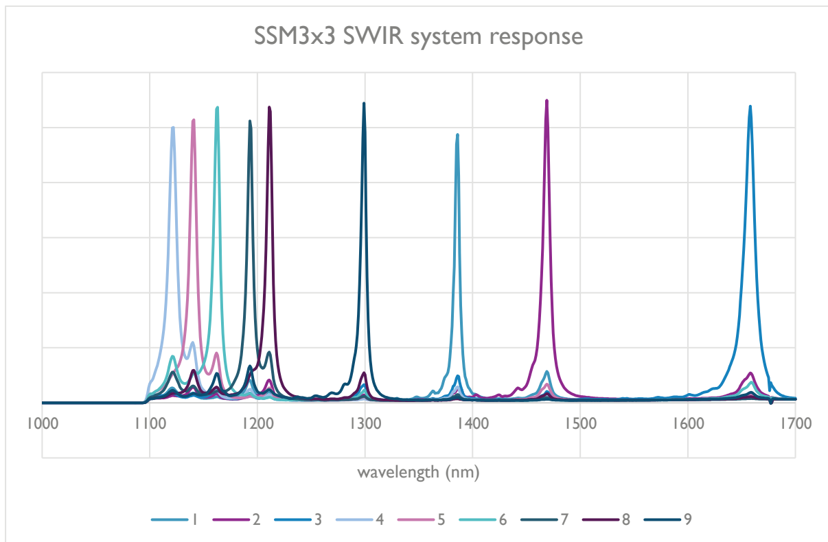
Figure 1. Example of a snapshot SWIR system response graph
