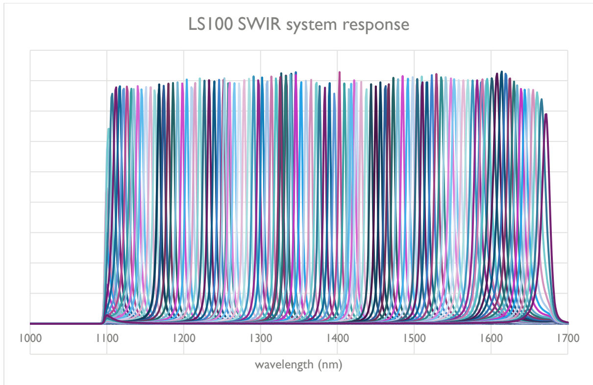
Figure 1. Example of a linescan SWIR system response graph
